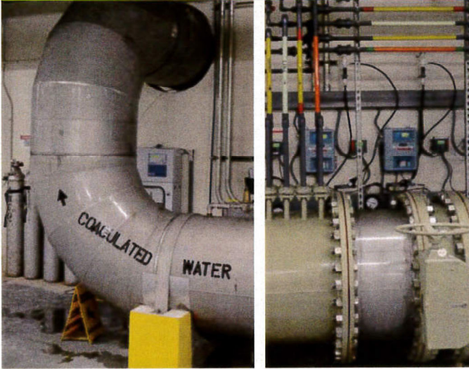
Mixing and Coagulation
